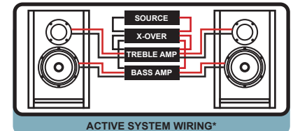
ACTIVE SYSTEM WIRING*
